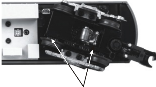
Grease Idler Gears (G)
